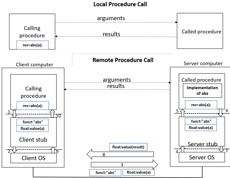
Figure 1: The mechanism of the Remote Procedure Call and the Local Procedure Call
